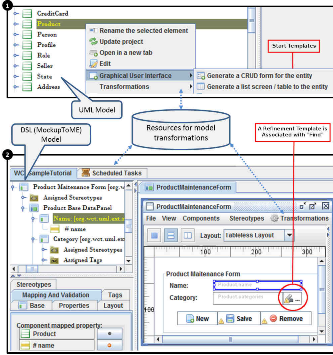
Figure 7: Screen-shots of models and start templates.
