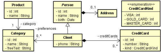
Figure 6: Conceptual model designed manually with the Astah UML tool. This is a logical view of the Model layer, illustrated as part of the scenario associated with the use case view shown in Figure 2.
