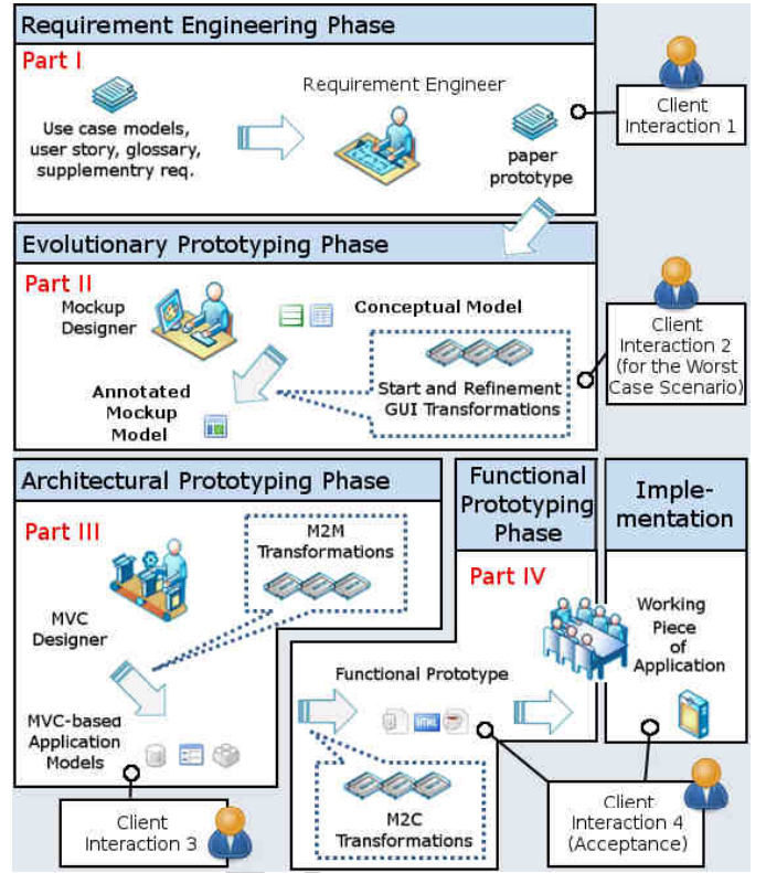
Figure 10: Overview of steps proposed for rapid application prototyping in four interactions with client in the MockupToME Method.
