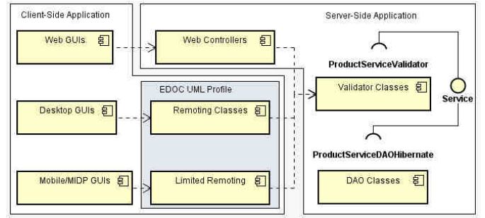
Figure 20: Component diagram describing the architecture.
