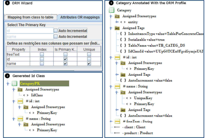
Figure 19: Entity layer annotated with the ORM Profile with the help of a wizard.
