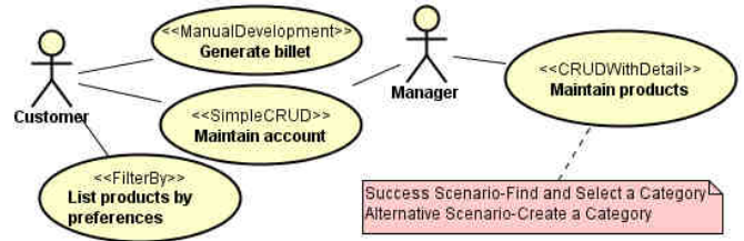
Figure 2: E-commerce use cases designed manually conforms to the CRUD UML Profile. This is a use case view that illustrates a functionality considered for implementation in a unique iteration of the software development process.
