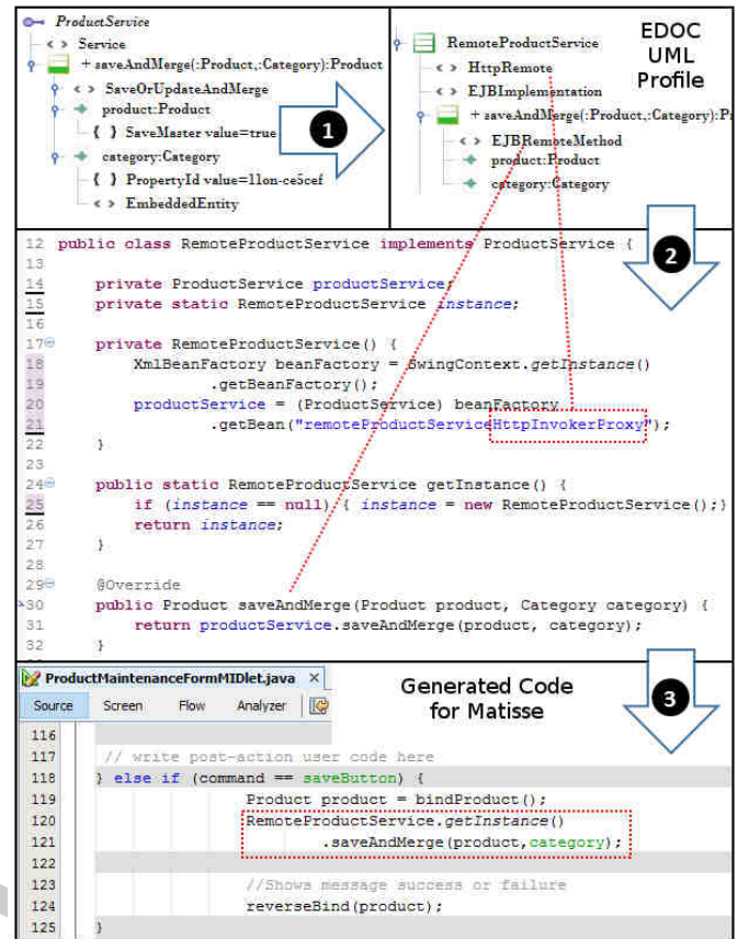
Figure 28: Generated source code for the Remote layer in HTTP Remote.
