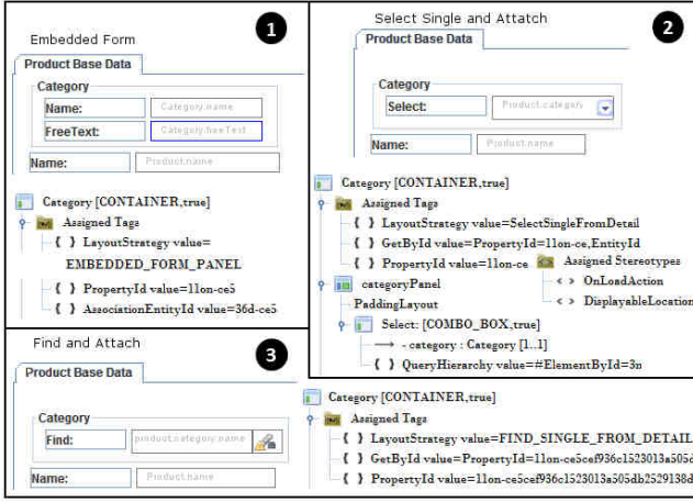
Figure 15: Layout strategies for 0..1 relationships.
