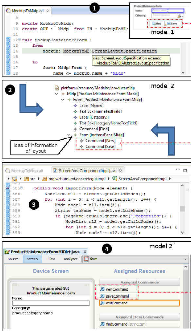
Figure 27: Generated models for the View layer on a mobile device dependent from the CLDC platform: the source code in (1) allows the generation of a model conforms to Mobile DSL shown in (2) and; the source code in (3) allows to import/export such model for the XML file associated with the Matisse (Mobile Designer) shown in (4).
