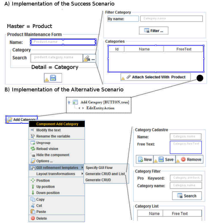
Figure 16: Implementation of scenarios for the use case Maintain Products .
