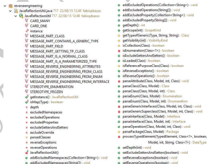
Figure 30: The class developed for automatic reverse engineering.
