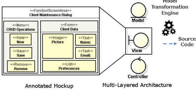
Figure 5: Illustration of an annotated mockup, manually designed in the Astah UML modelling tool with stereotypes from the GUI Profile [28] and our extensions from Action Profile, as part of the view layer of a multi-layered architecture based on MVC.
