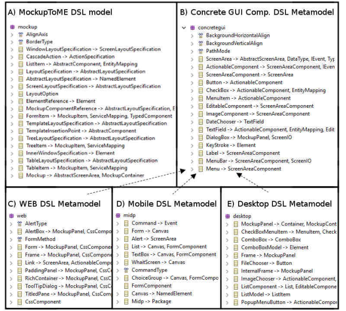
Figure 4: DSLs for representation of the View layer in different abstraction levels.
