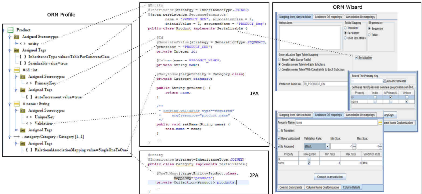
Figure 22: Generated source code for the Model layer implemented with JPA (2.0).
