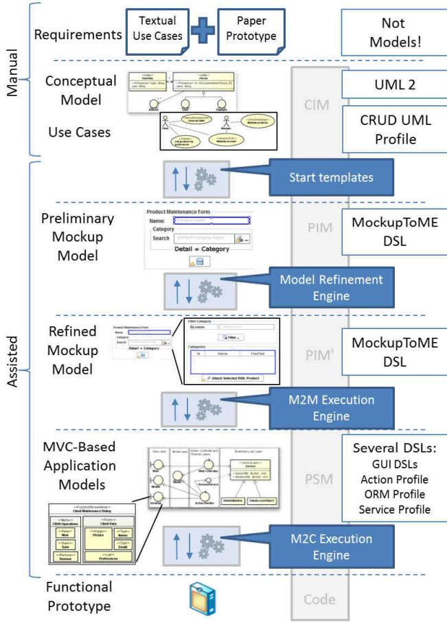
Figure 3: Model transformation lifecycle adopted in the automated design approach.
