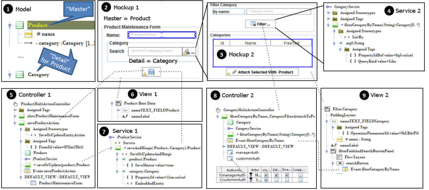
Figure 17: Design elements represented through the methodology in support for the use case Maintain Products.
