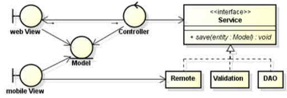
Figure 9: Structures for multi-layered application based on MVC.
