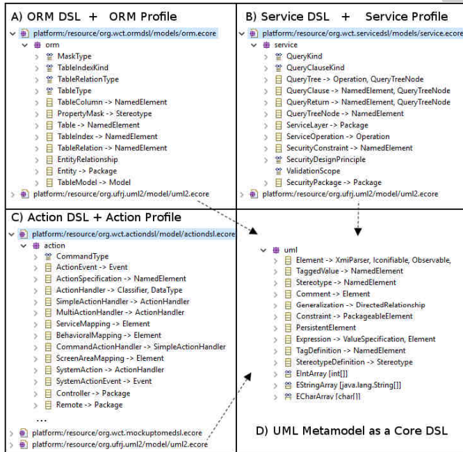
Figure 8: Metamodels for the representation of MVC-based Application Models.
