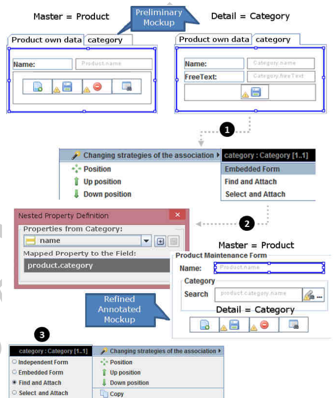
Figure 14: Steps to refine annotated mockups: changing refinement strategies to handle associations.
