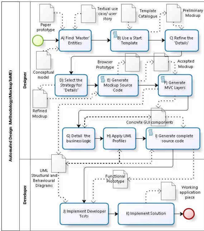
Figure 11: MockupToME Method with tasks assisted by tool, allowing the generation of models in different abstraction levels.
