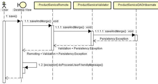
Figure 18: Message call to process the action saveAndMerge in the underlying multi-layered architecture.
