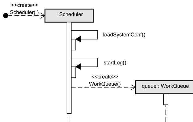
Figure 8: Initialising the Runtime System.
